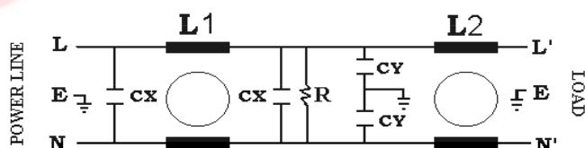
AC circuit (Two-stage)
