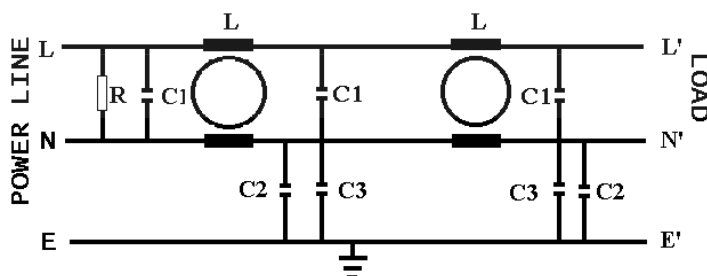
AC circuit (two-stage)
