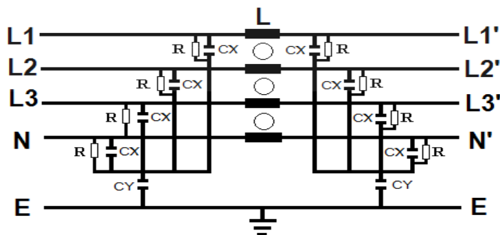
AC circuit (One-stage)
